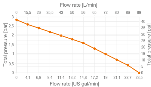
Dispensing volume submersible pump CENTRI SP80
