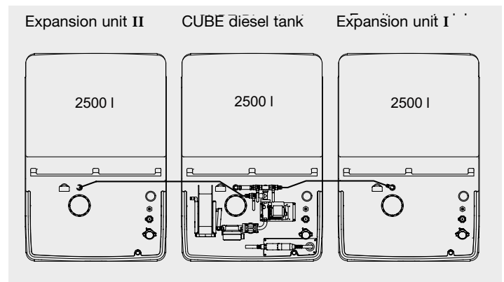
CUBE diesel refuelling system 7,500 L with expansion unit I and II
