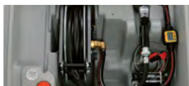
440 L Premium with automatic nozzle and meter
